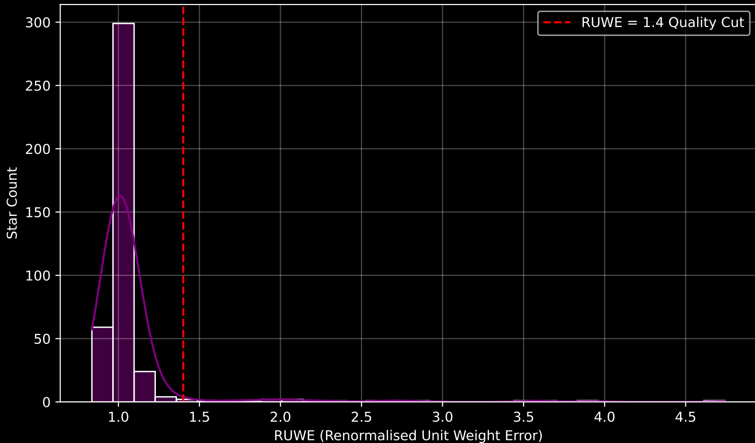
GAPOGEE DR17 Field [090-04] RUWE Distribution (n= 404)
