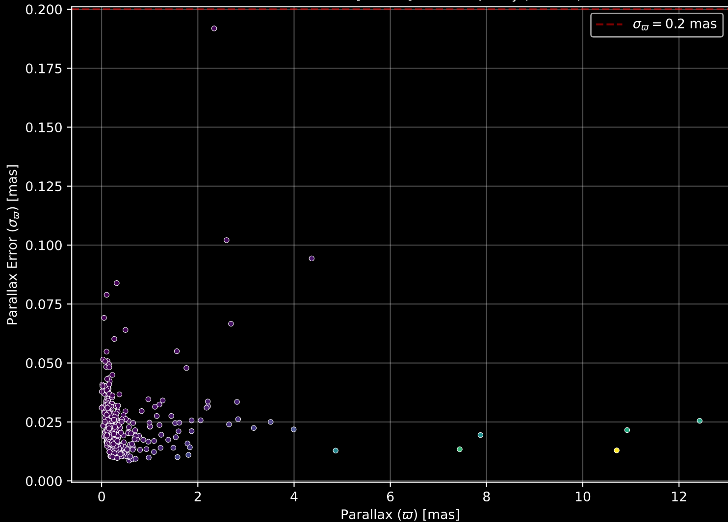
APOGEE DR17 Field: [090-04] Parallax Quality (n= 406)
