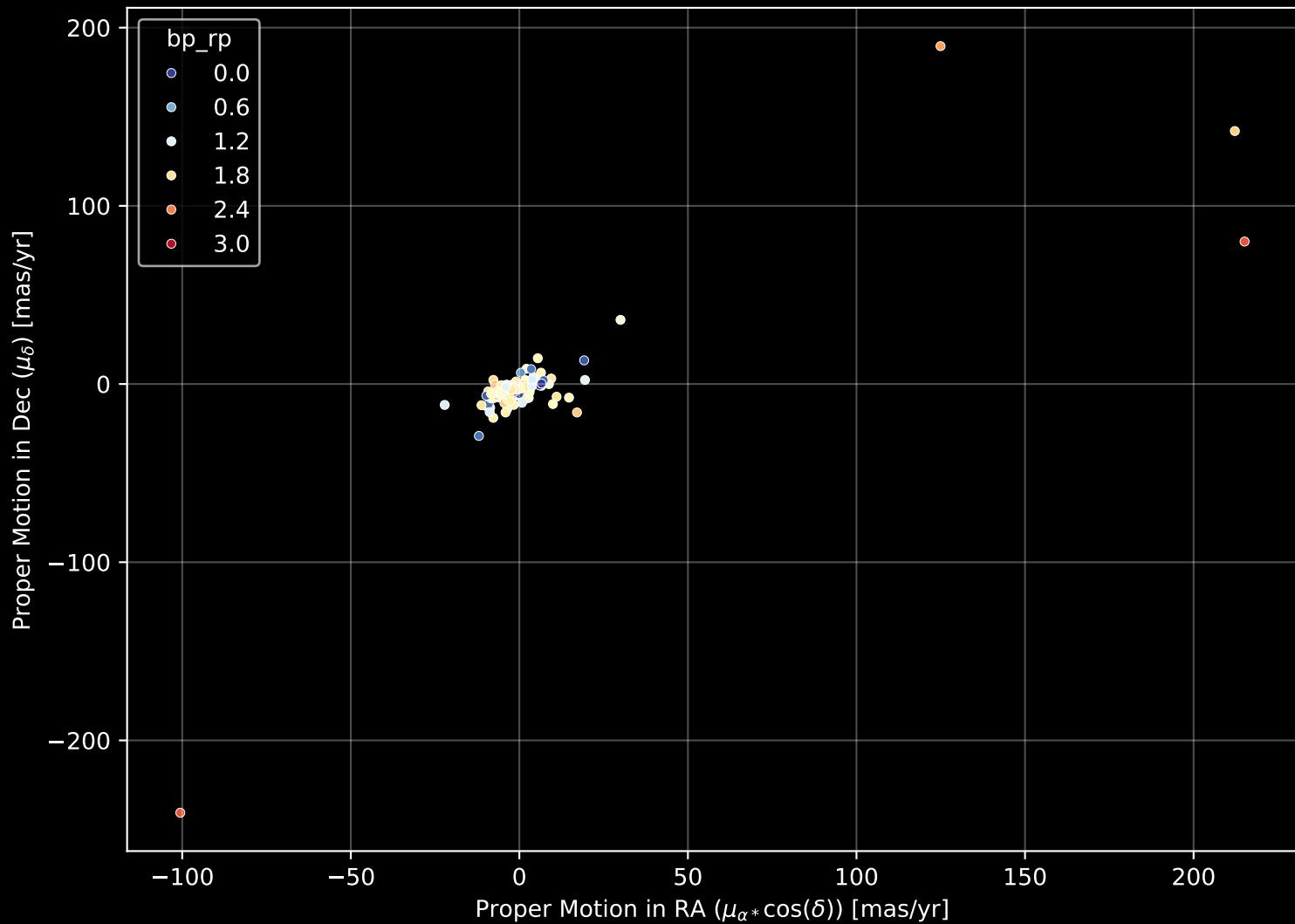
APOGEE DR17 Field: [090-04] Proper Motion Diagram (n= 406)
