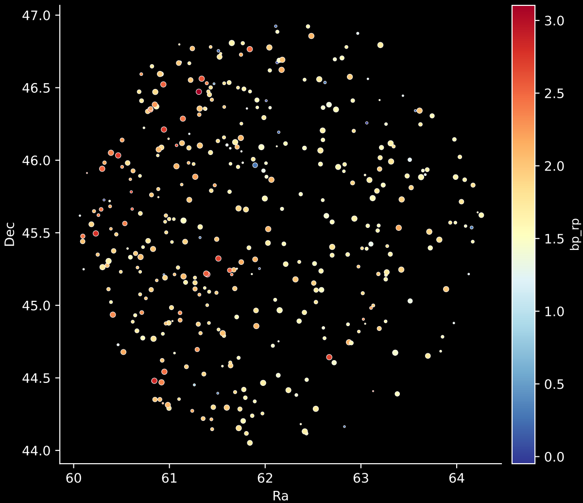
APOGEE DR17 Field: [090-04] Stars: 406
