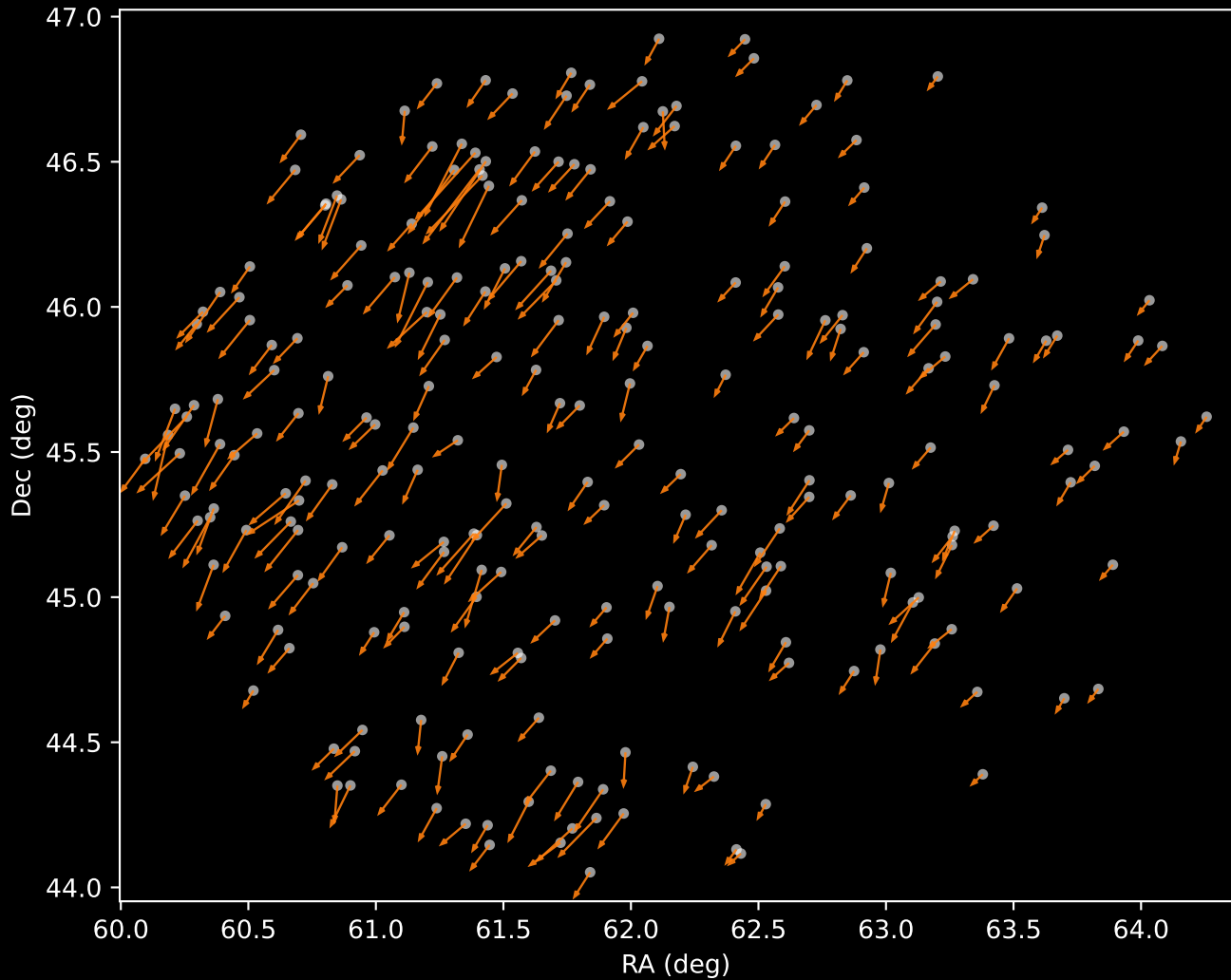
APOGEE DR17 Cluster 2 Proper Motion Vectors (n=241)
