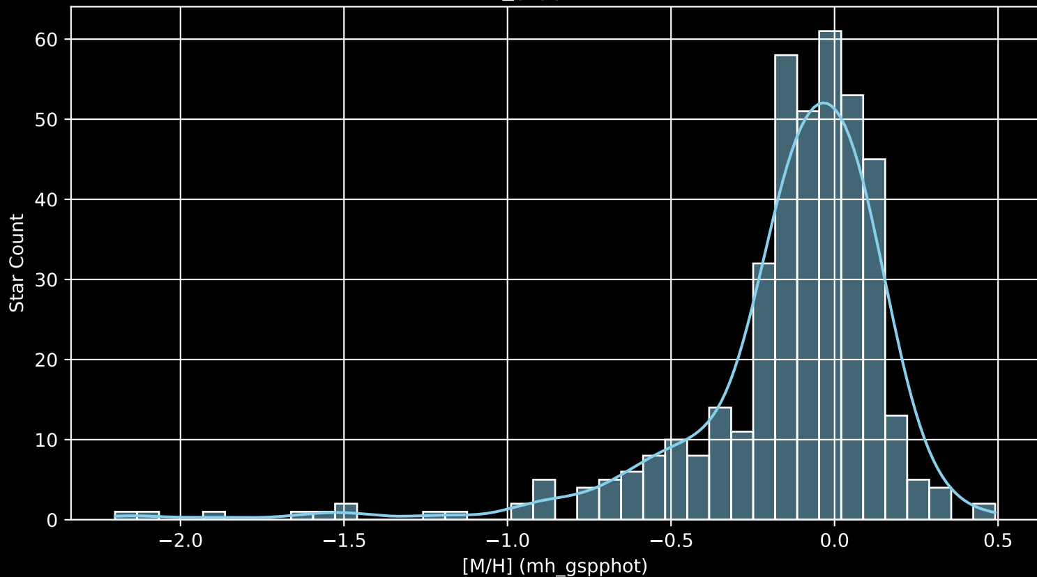
APOGEE DR17 Field: [090-04 [M/H] (mh_gspphot) (n= 406)
